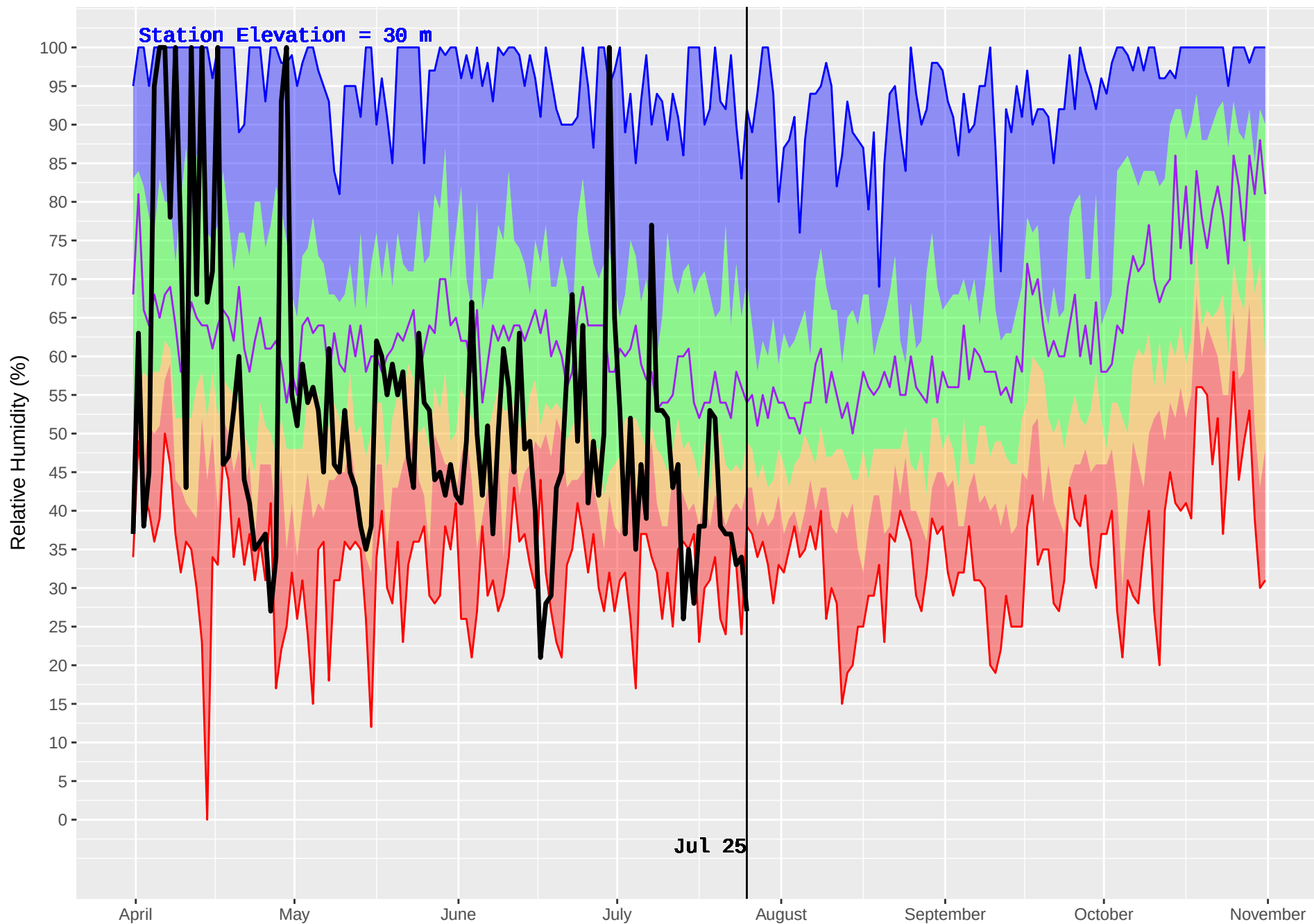
CEDAR (59) : Historical (1989–2016) and Current (2018) Noon Relative Humidity
