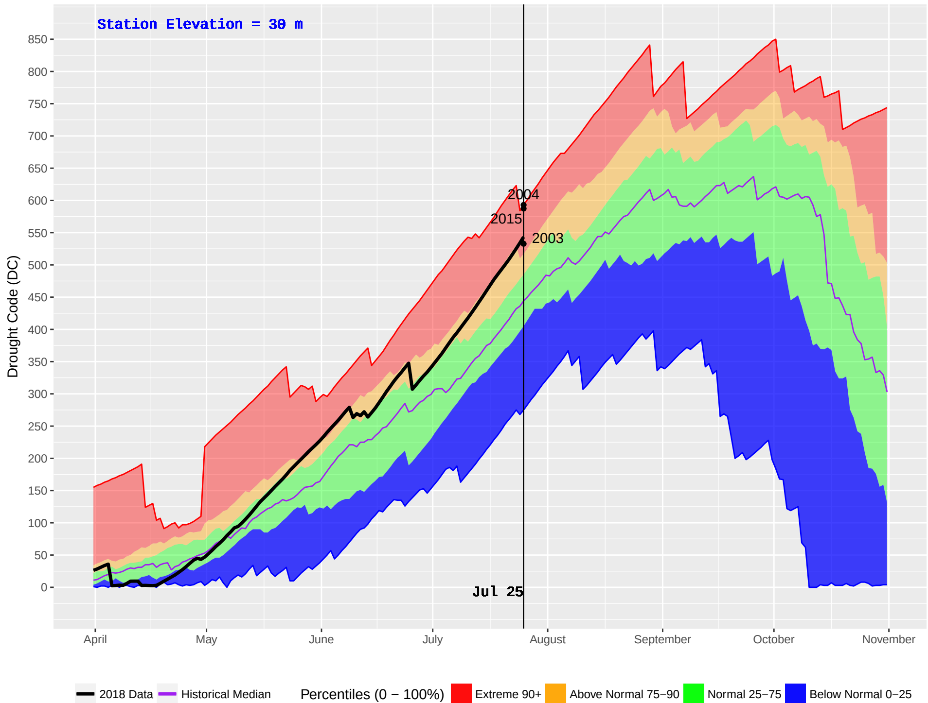
CEDAR (59) : Historical (1989–2016) and Current (2018) Noon Drought Code (DC)
