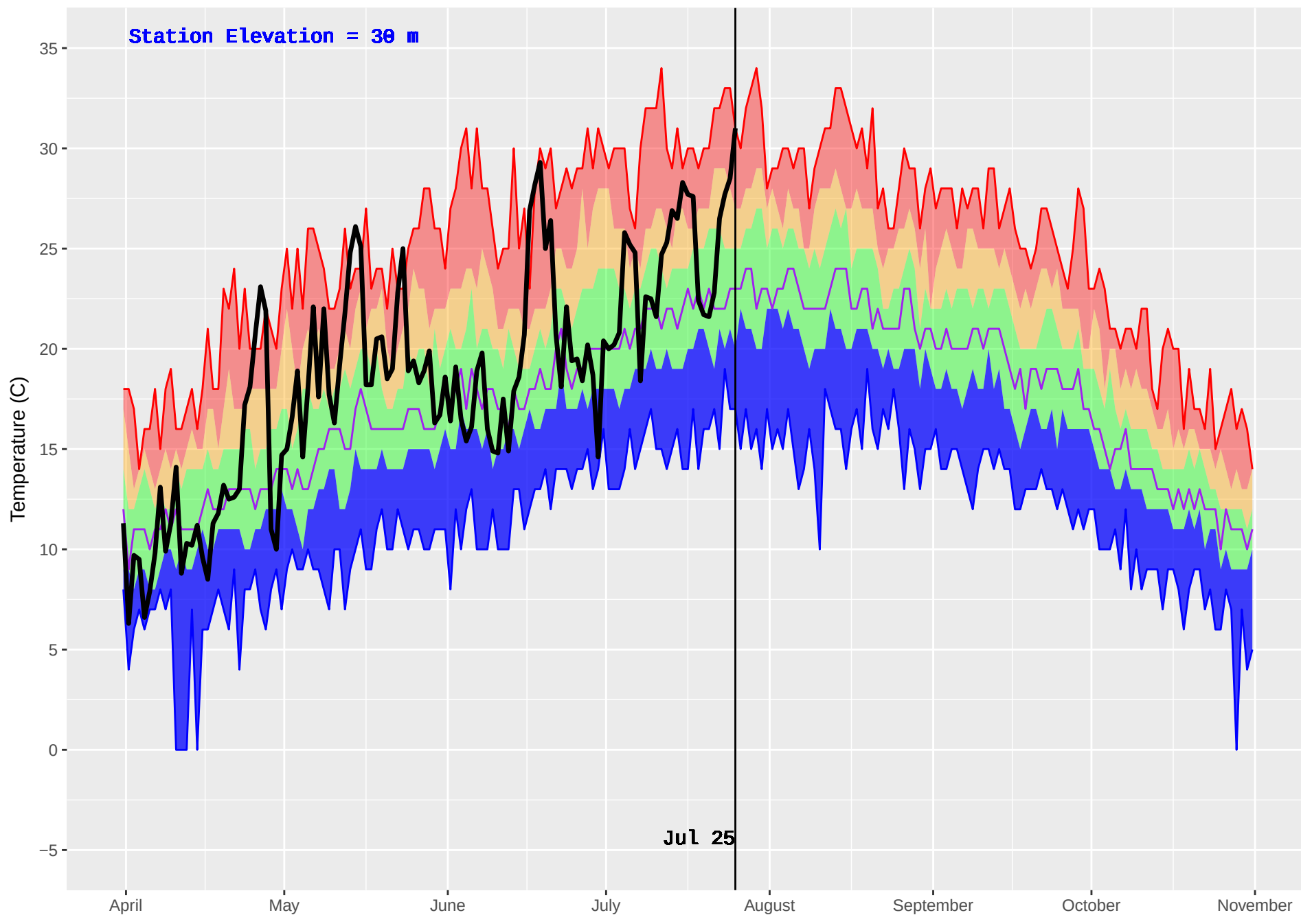
CEDAR (59) : Historical (1989–2016) and Current (2018) Noon Temperature
